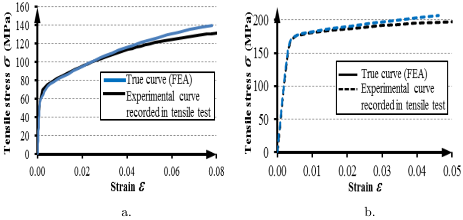
Figure 8. Comparison of the true and experimental stress-strain curves recorded in tensile tests for a. EN AW-6060-T4 aluminum alloy; b. EN AW-6060-T6 aluminum alloy
