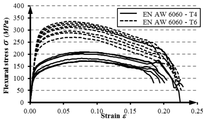
Figure 5. Stress strain curve ( \sigma - \varepsilon ) recorded in the three point bending test
