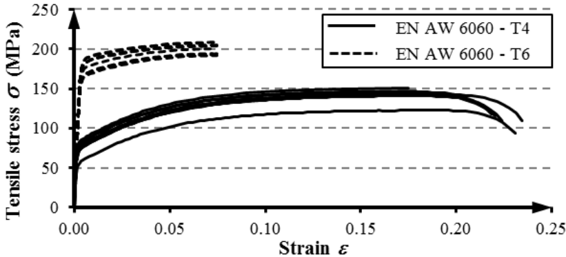
Figure 4. Stress strain curve ( \sigma - \varepsilon ) recorded in the tensile test
