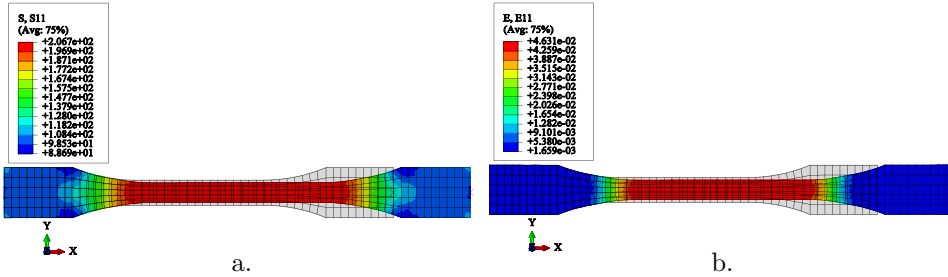
Figure 7. FEA results for material properties EN AW-6060-T6 aluminum alloy: a. Stress; b. Strain
