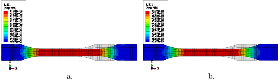
Figure 6. FEA results for material properties EN AW-6060-T4 aluminum alloy: a. Stress; b. Strain
