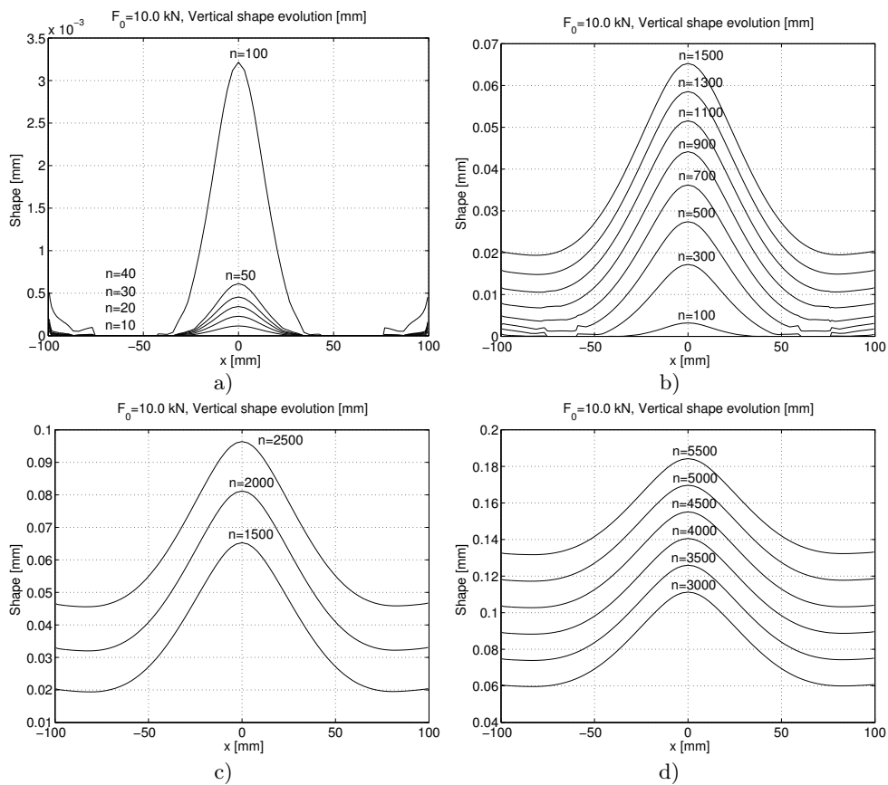
Figure 13. Evolution of contact shape in the wear process.
