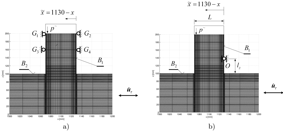
Figure 2. Periodic sliding on the contact interface between punch and strip. The number of finite elements in body 1 along the x direction is 8, and in vertical z direction is 7. The lines are drawn through the Lobatto integral coordinates.
